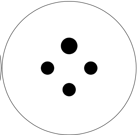
15A Walsall Gauge 'A' 4 pin
