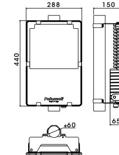
Horizontal pole mounting
