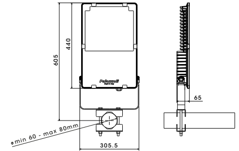
Horizontal pole mounting
