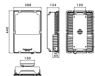
Ceiling mounting
