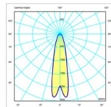
Symmetrical 18^{\circ} narrow beam
