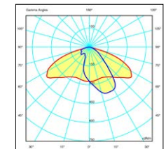
Roadway 65^{\circ} wide beam
