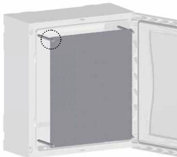
SPACERS + BACK PLATE Back plate adjustable in depth using the spacer
